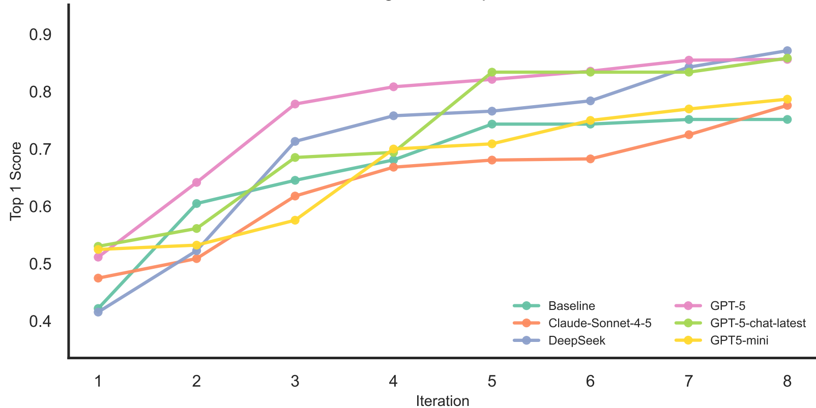
Convergence of Top 1 Score
