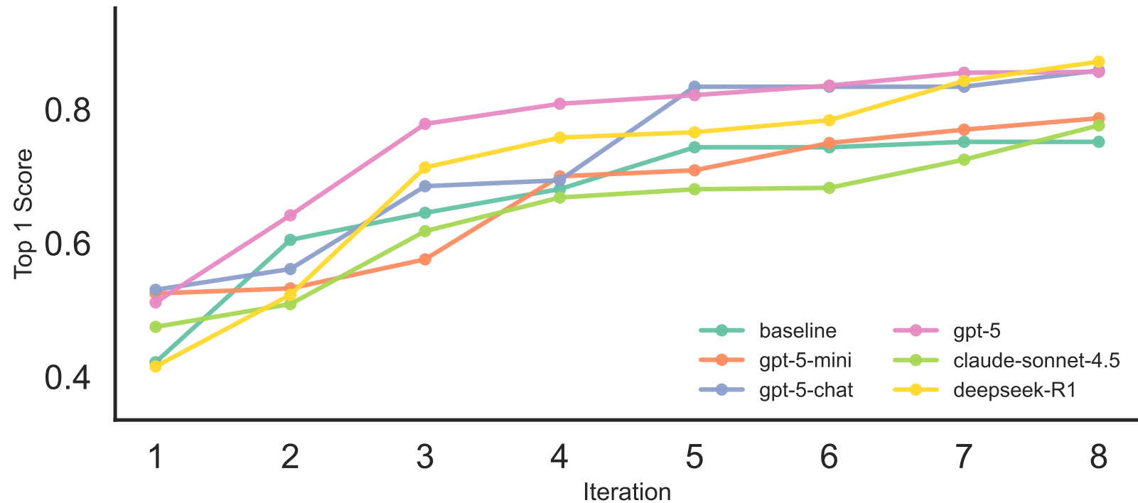
Convergence of Top 1 Score
