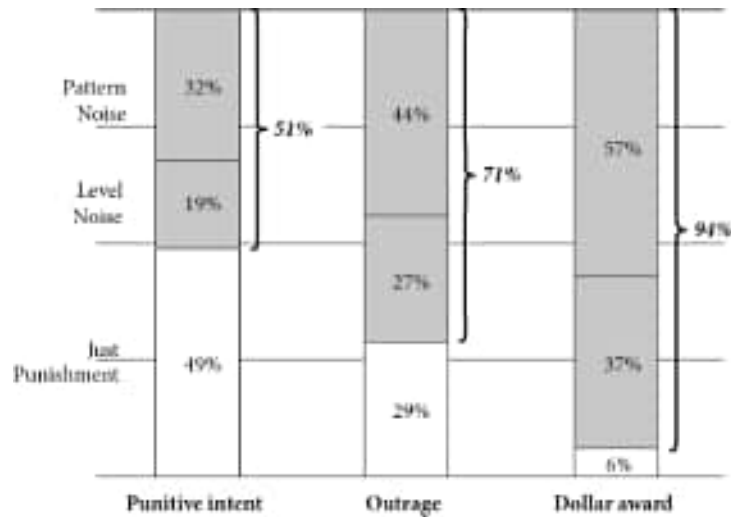
FIGURE 13: Components of judgment variance
