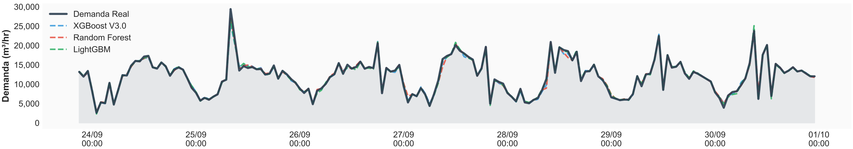
XGBoost V3.0 vs Demanda Real
