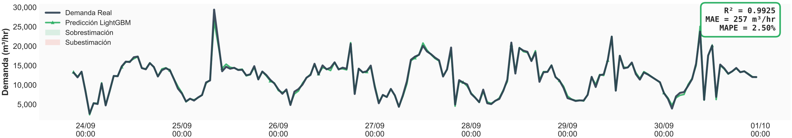
LightGBM vs Demanda Real
