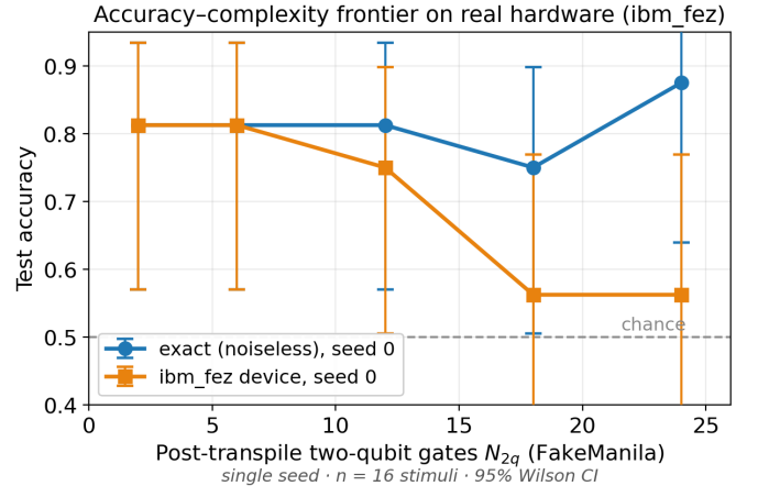
Fig. 4. The accuracy-complexity frontier on a physical IBM device (ibm_fez, hard task, 16 test stimuli, single seed; bands are 95% Wilson intervals). The exact curve stays high while the device curve falls with N_{2q} , collapsing toward chance for the full circuit. The widening gap between the curves is the cost of redundant entangling capacity on real hardware—and the case for compression.
