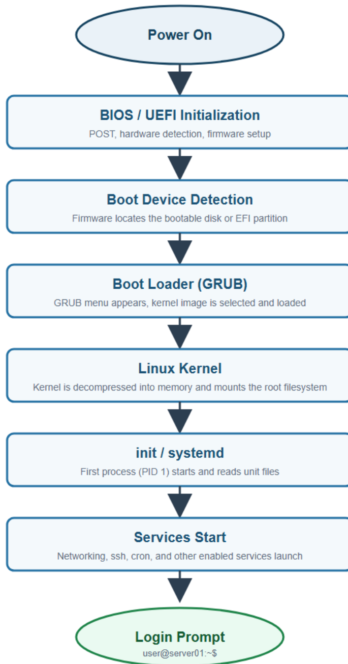
Figure 1. Sequence of events from power-on to the login prompt on Ubuntu Server.
