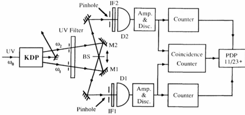
Figure 3.3: Set-up.
