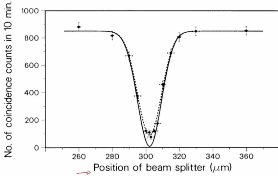
Figure 3.5: Coincidence rate as a function of the relative delay \Delta\tau . The dip at zero delay is a signature of two-photon interference.
