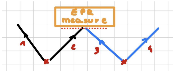
Figure 3.12: Scheme of entanglement swapping in a quantum repeater.
