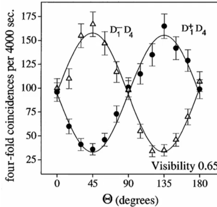
Figure 3.13: Coincidence rates for entanglement swapping.
