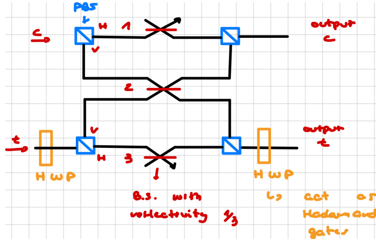
Figure 3.16: C-NOT gate through p.B.S.s, u.B.S.s, and H.W.P.s.
