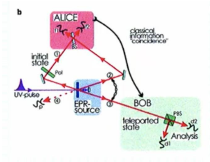
Figure 3.11: Experimental setup for teleportation of the Innsbruck group.
