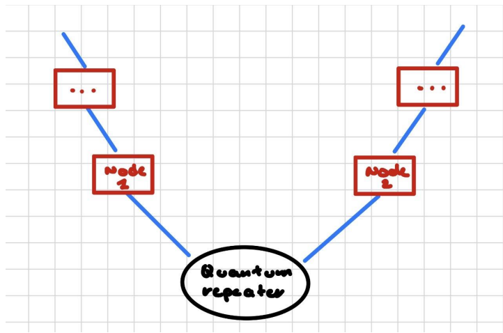
Figure 3.14: Entanglement swapping in a quantum repeater.
