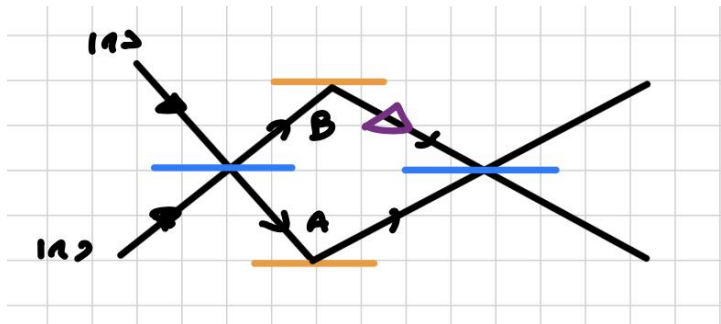
Figure 3.7: Path-entangled photons
