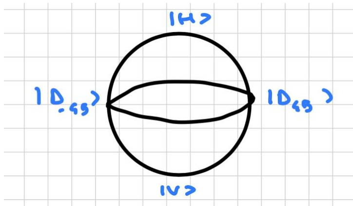
Figure 3.9: Poincaré sphere
