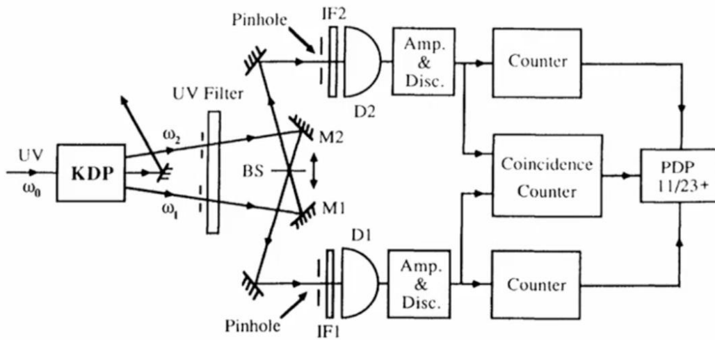
Figure 3.4: Hong-Ou-Mandel interference set-up.
