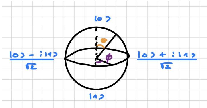
Figure 3.8: Bloch sphere
