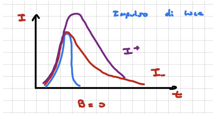
Figure 1.1: B = 0
