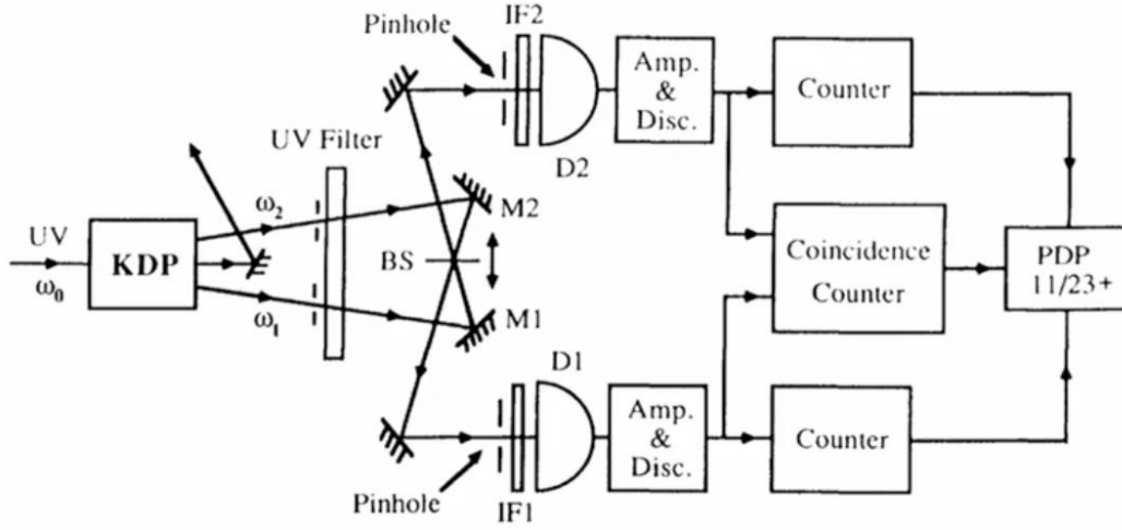
Figure 3.4: Set-up.
