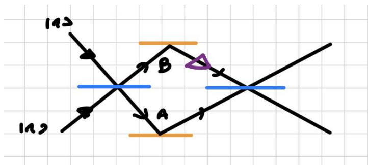
Figure 3.7: Path-entangled photons
