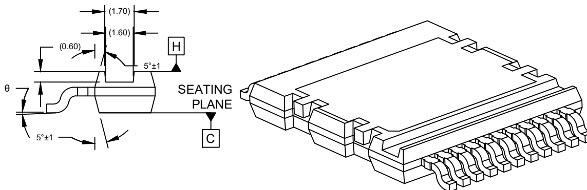
DETAIL B
