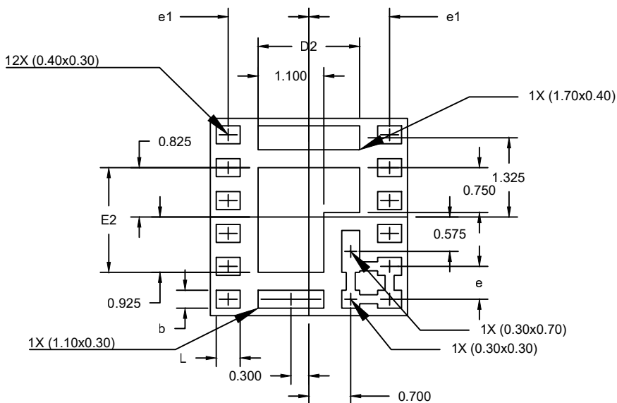
BOTTOM VIEW
