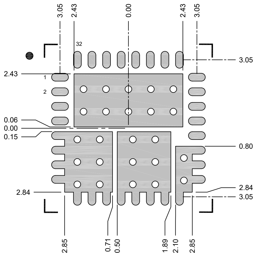
RECOMMENDED LAND PATTERN SEE SHEET 2 FOR ADDITIONAL DIMENSIONS
