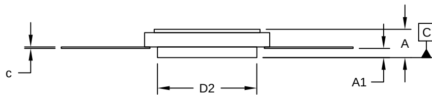
END VIEW
