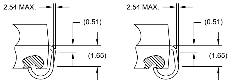
DETAIL C
