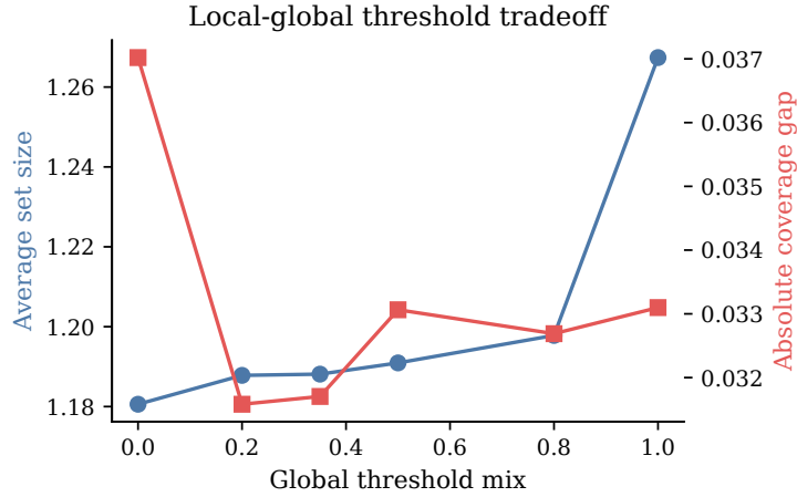
Figure 4: Ablation of the local-global threshold mix on five datasets. Intermediate mixing recovers coverage relative to purely local thresholds while retaining smaller prediction sets than the global augmented threshold.
