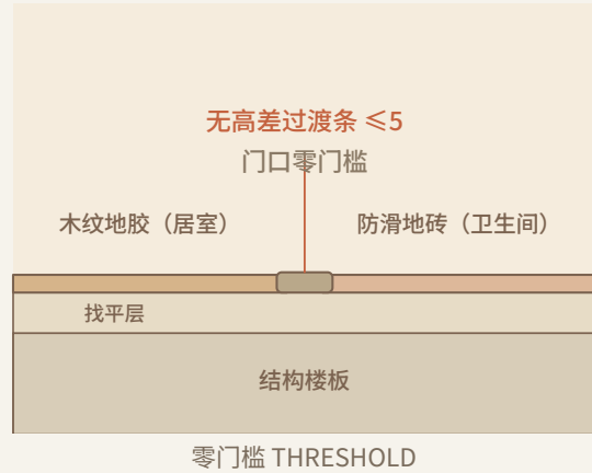
零门槛 THRESHOLD
