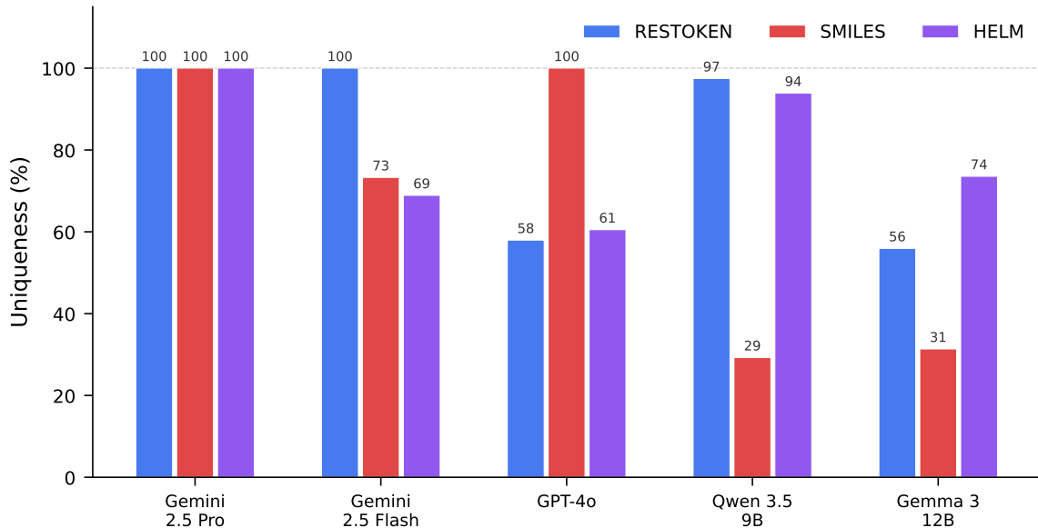
(b) Sequence Diversity (Unique / Total)
