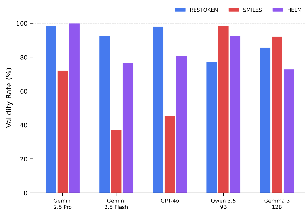
(a) Zero-Shot Validity
