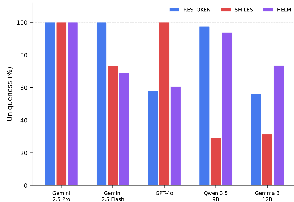
(b) Sequence Diversity
