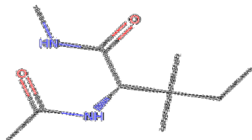
α-amino acid (isoleucine analog)
