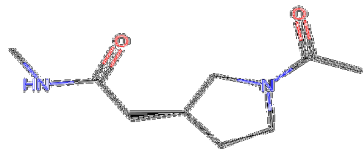
γ-amino acid (γ-proline analog)
