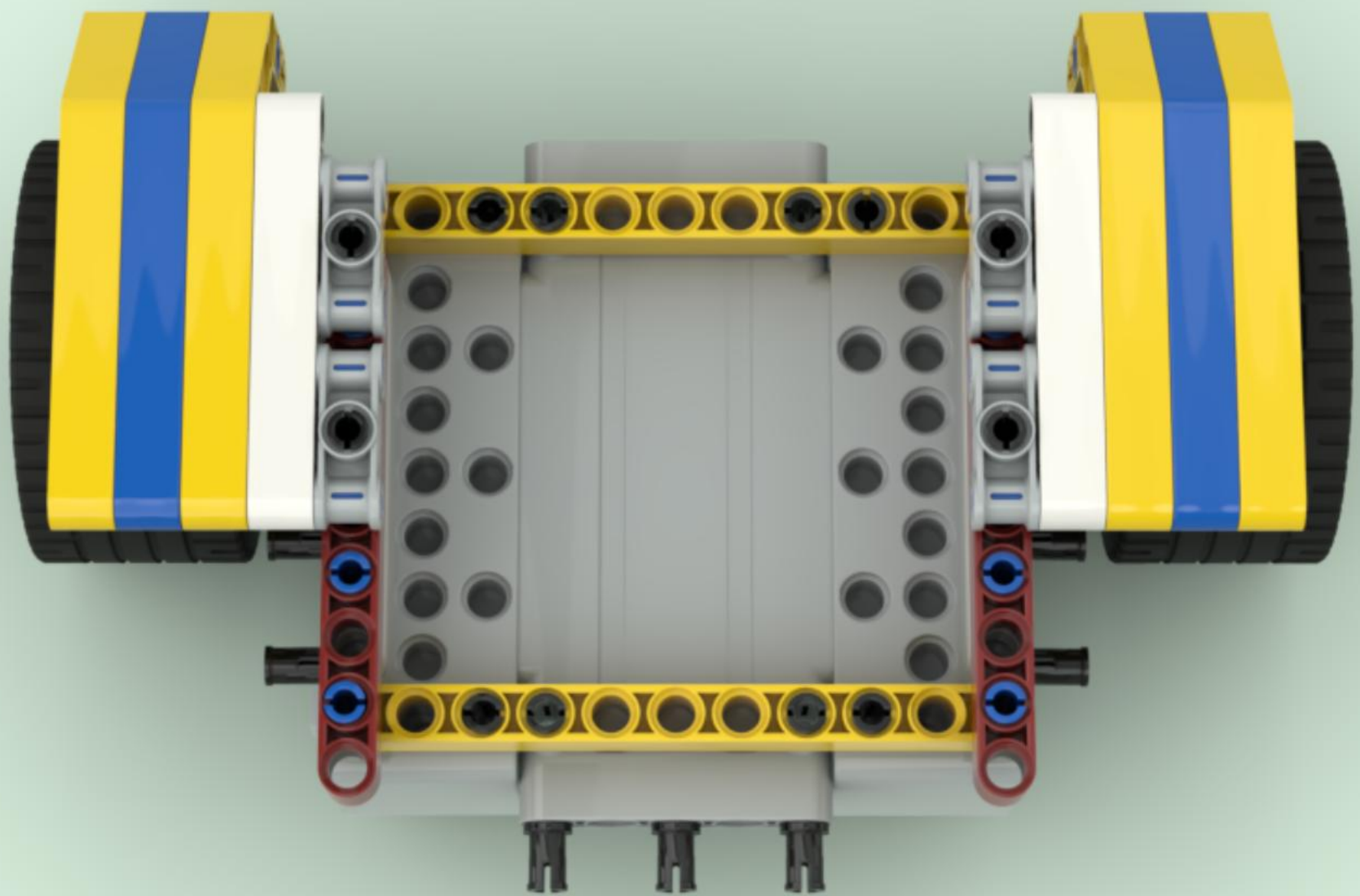
Motor Parts
