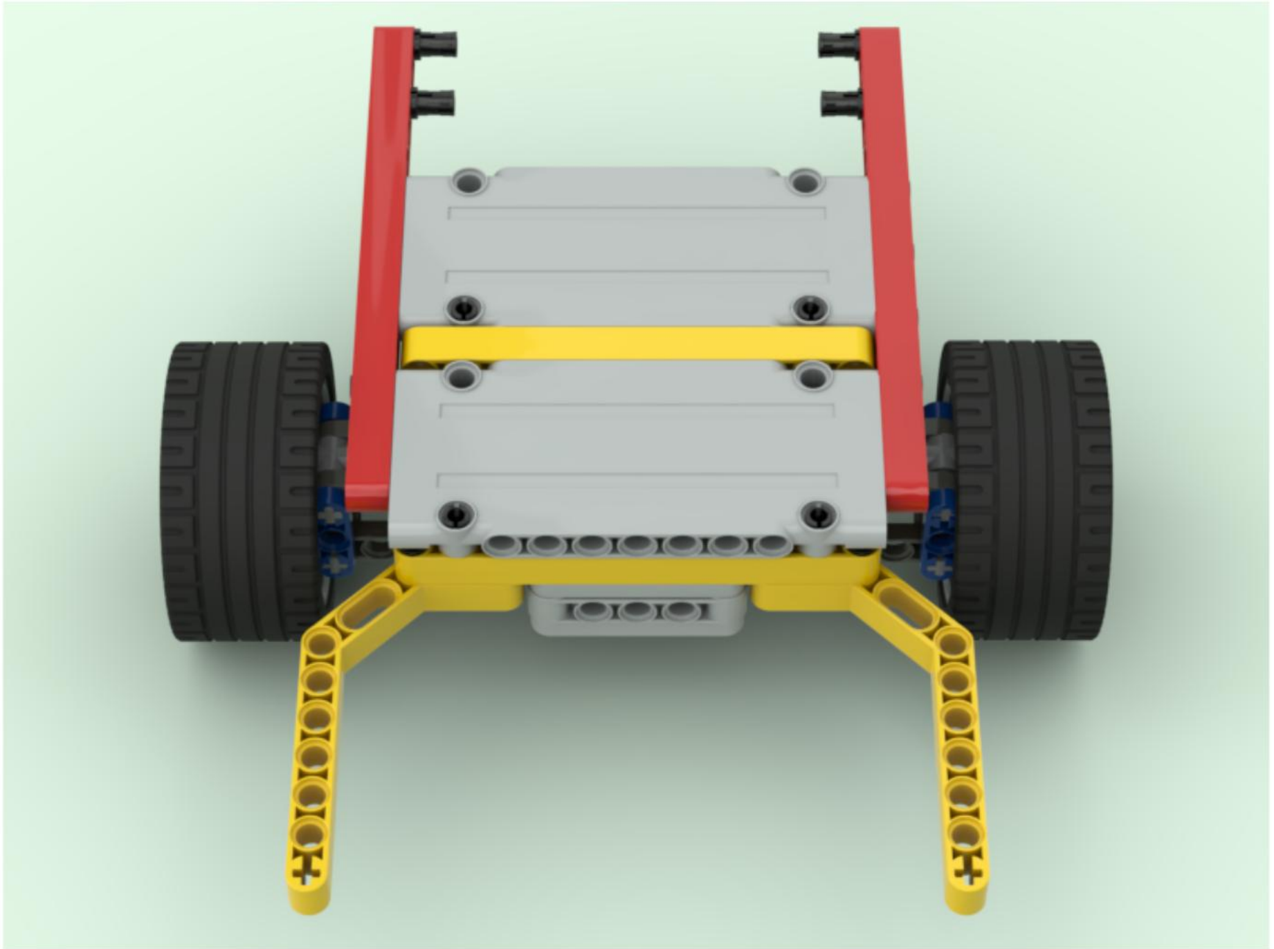
Front Wheels
