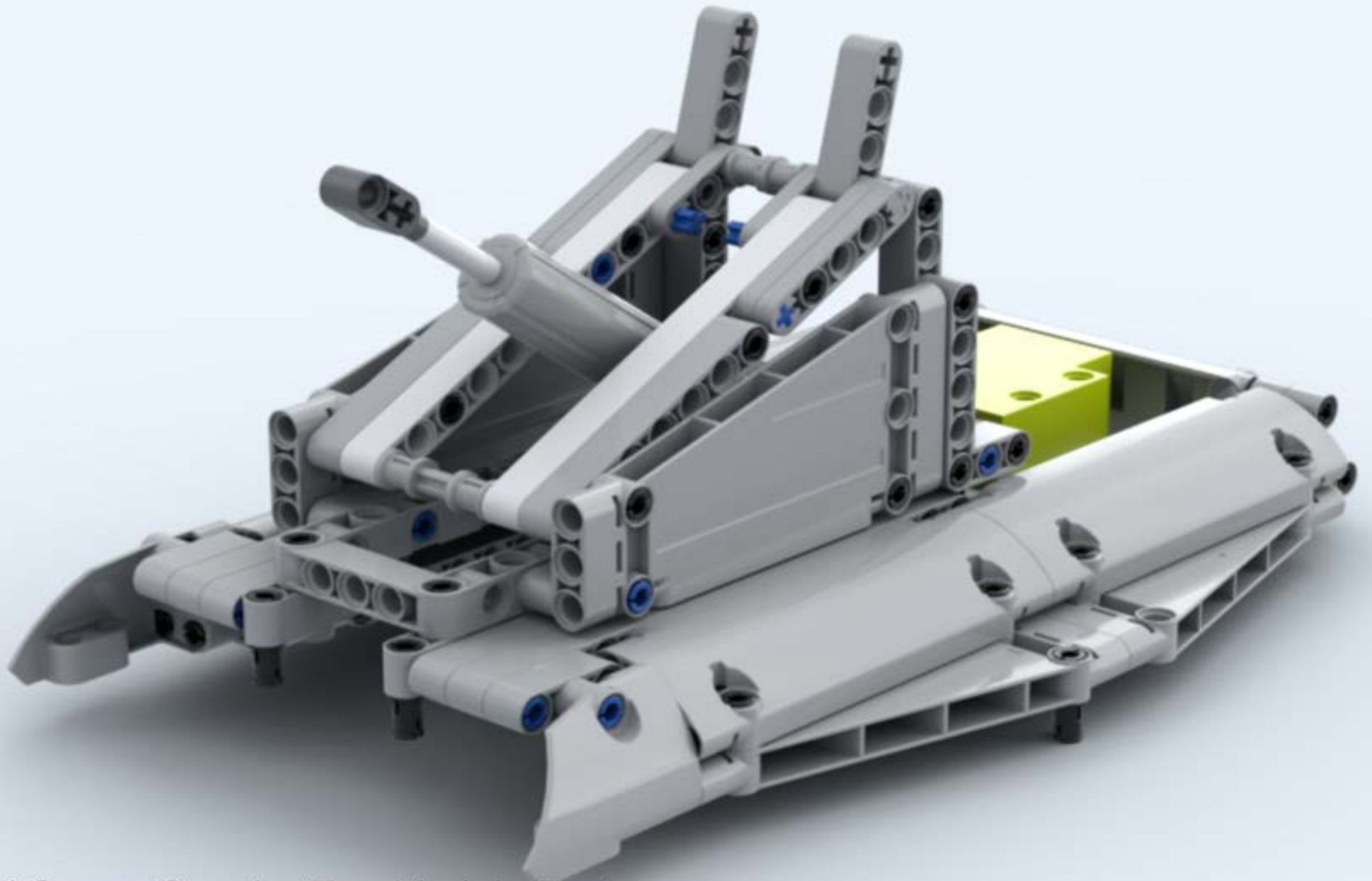
AI Space Crawler Top Module Parts Deign by Lewis Ng
