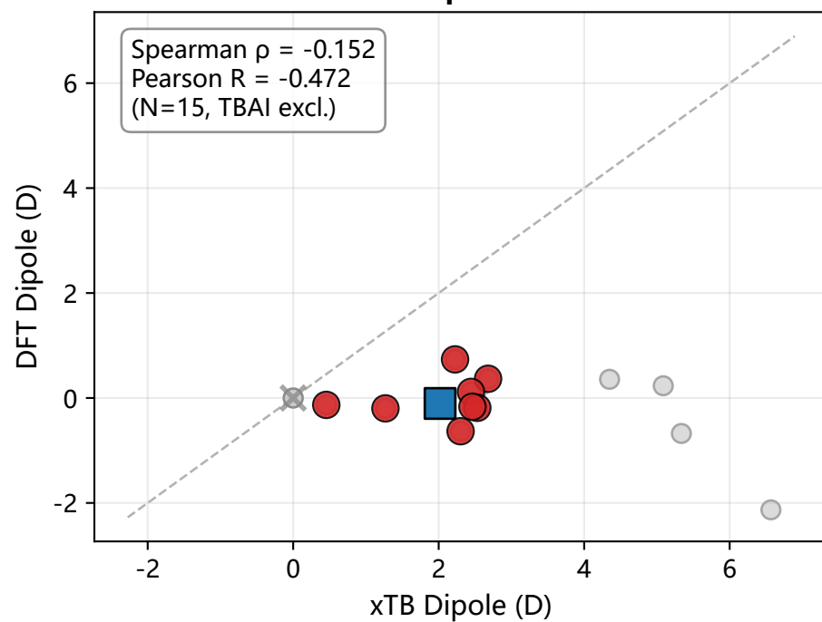
Dipole
