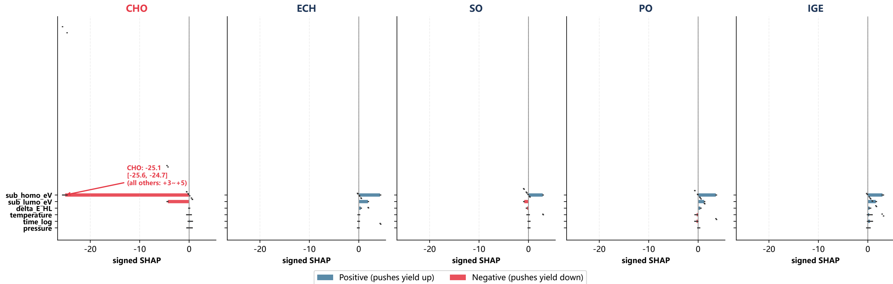
Fig. 4 | Per-Substrate Top-5 Signed SHAP with 95% CI (100 Bootstrap)
