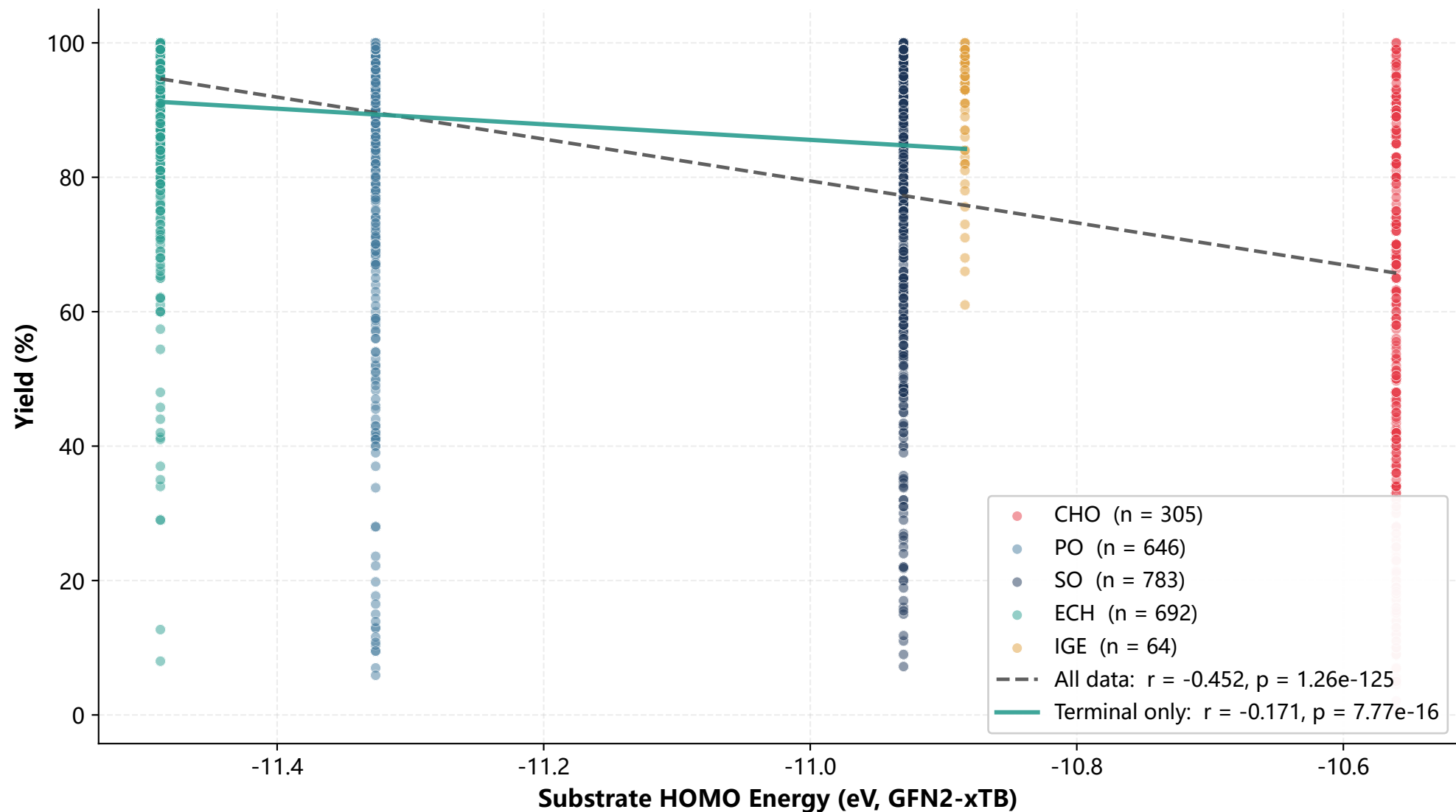
Fig. 5 | Substrate HOMO vs Yield: CHO Drags Down Global Correlation (gap 2.7x)
