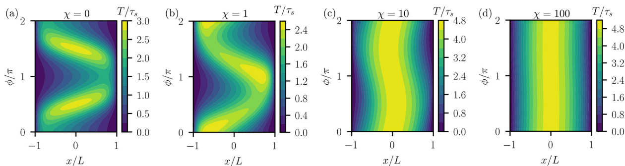
Fig. 4 Contour plots showing the MFPT of CABPs in a 1D interval with absorbing boundaries as a function of the initial position ( x/L ) and orientation ( \phi/\pi ) for (a) \chi = 0 , (b) \chi = 1 , (c) \chi = 10 , and (d) \chi = 100 . In all cases, Pe = 10 and \beta = 0.1 .
