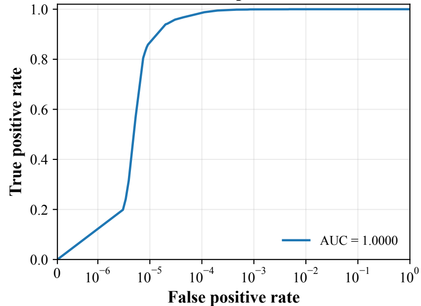
Full unordered pair-level ROC
