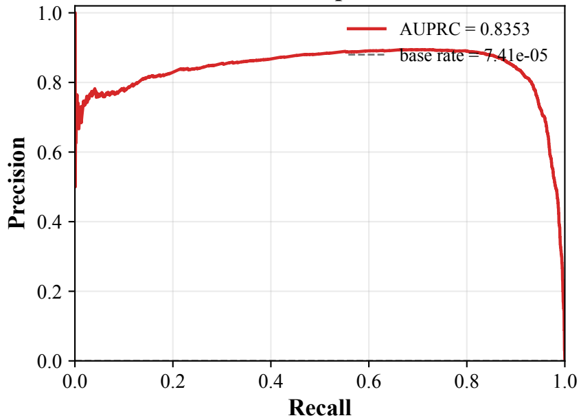
Full unordered pair-level PR
