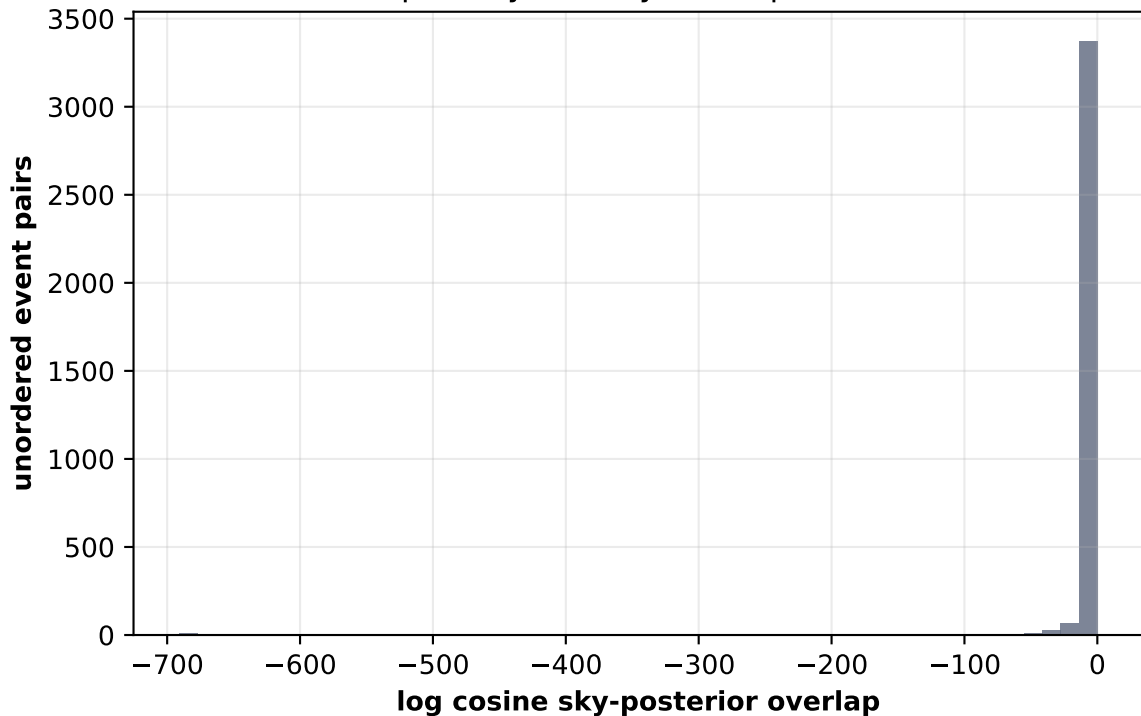
GWTC primary null sky-overlap distribution
