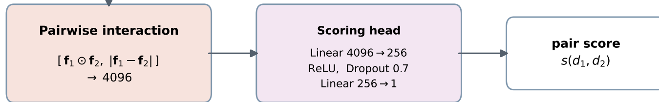
(b) Pairwise-interaction layer and scoring head
