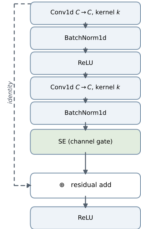
(c) Residual block
