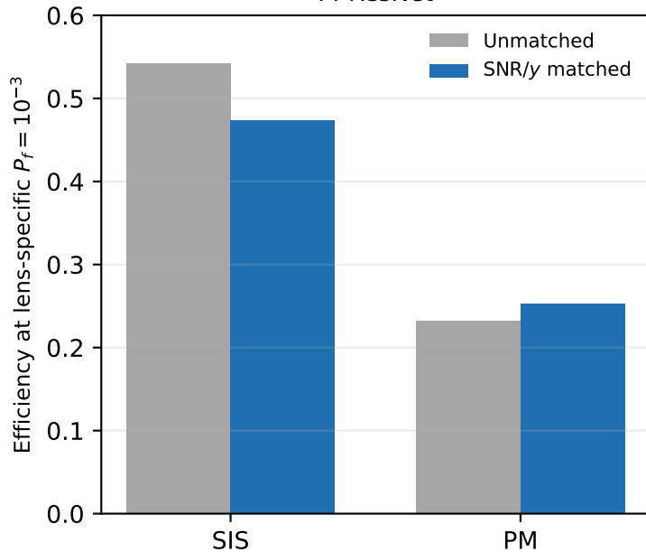
PI-ResNet
