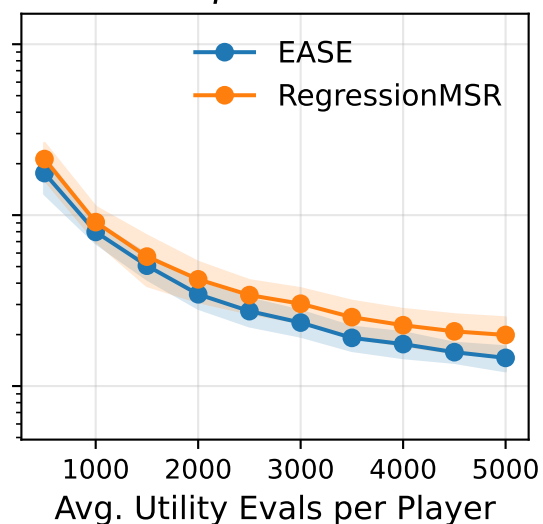
(e) EASE vs RegressionMSR, \eta = 0.75
