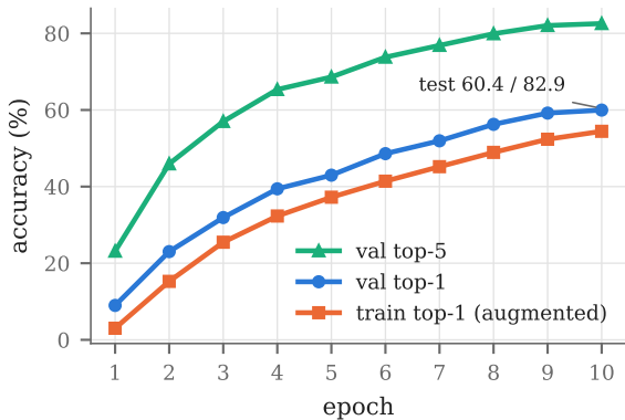
ResNet-36 + ArcGate, full ImageNet (650 classes), 2×A100
