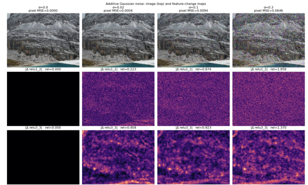
Figure 4. Qualitative noise test. Top: noisy images ( \sigma = 0, 0.02, 0.1, 0.3 ). Middle and bottom: per-location feature-change maps |\Delta| for relu1_2 and relu3_3 . The relu1_2 change is spatially uniform (it reacts to every noisy pixel). The relu3_3 change concentrates on textured regions such as the rock strata and the lake shore.
