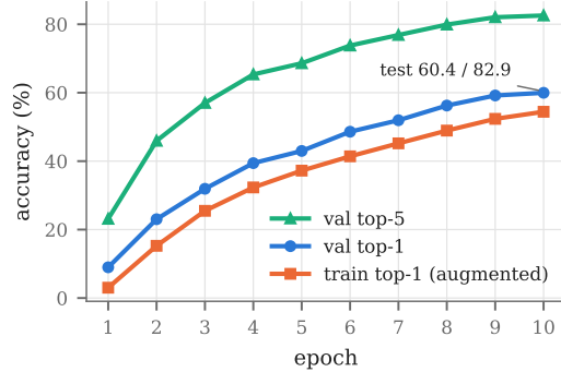
Figure 16. Full-ImageNet training curve (A100 run). Validation accuracy is still rising at epoch 10, and train accuracy (measured on augmented crops with label smoothing) stays below validation accuracy, so the model is not overfitting.
