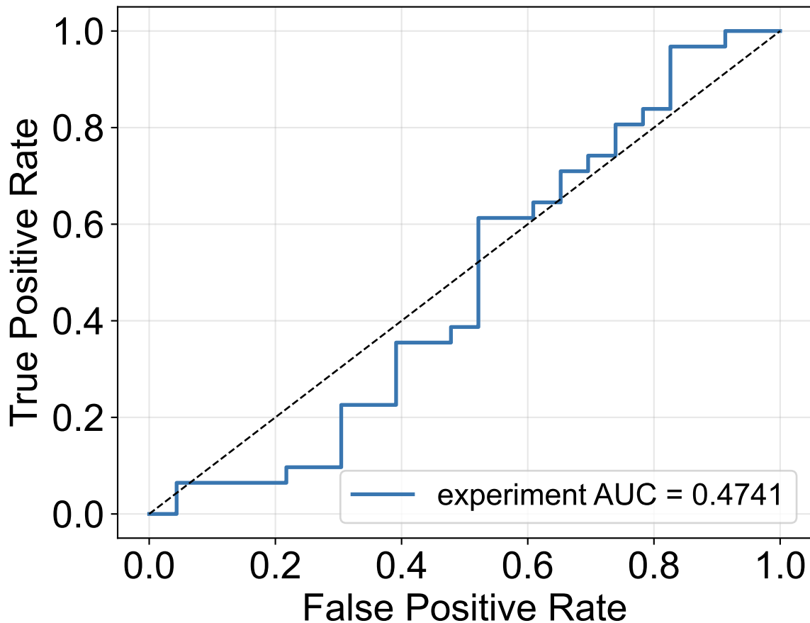
Cross-validated ROC Curve
