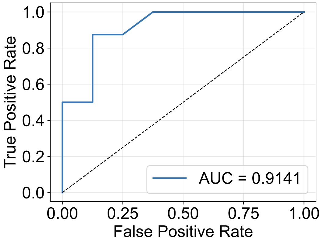
Cross-validated ROC Curve
