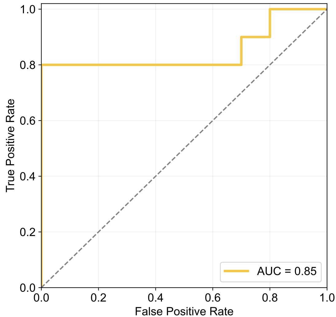
Test Set ROC Curve
