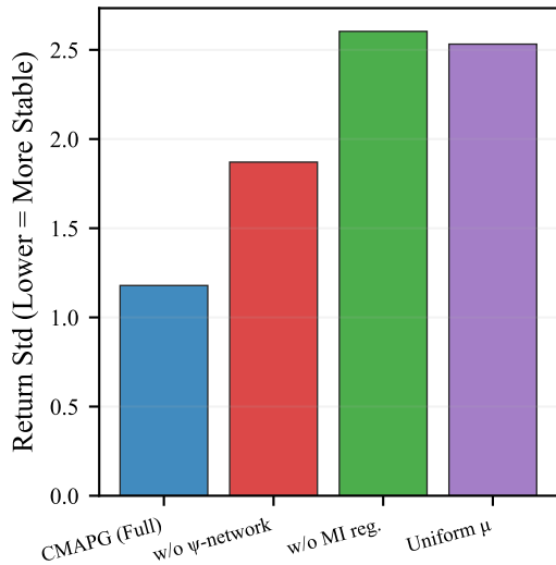
Training Stability
