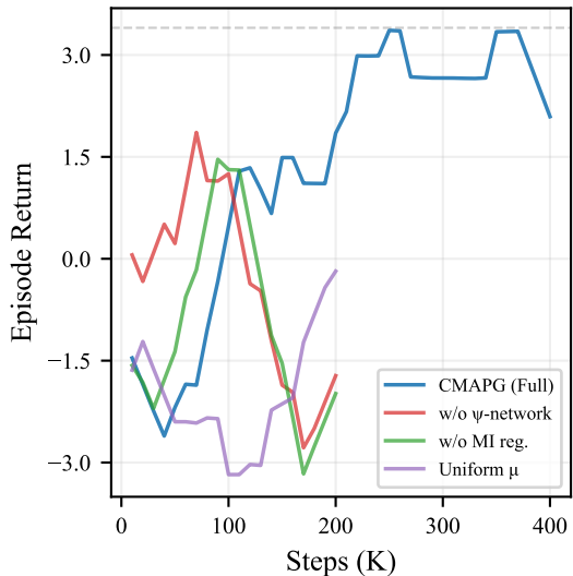
Ablation Learning Curves
