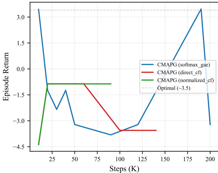
Advantage Mode: Learning Curves
