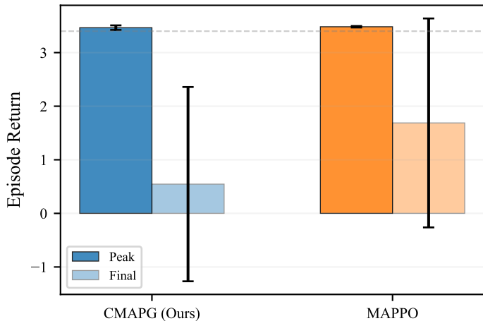
Peak vs Final (4 seeds, mean \pm std)
