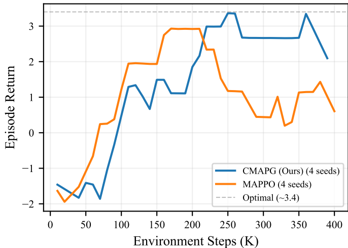
Learning Curves on Key-Lock (N=5, 4 seeds)
