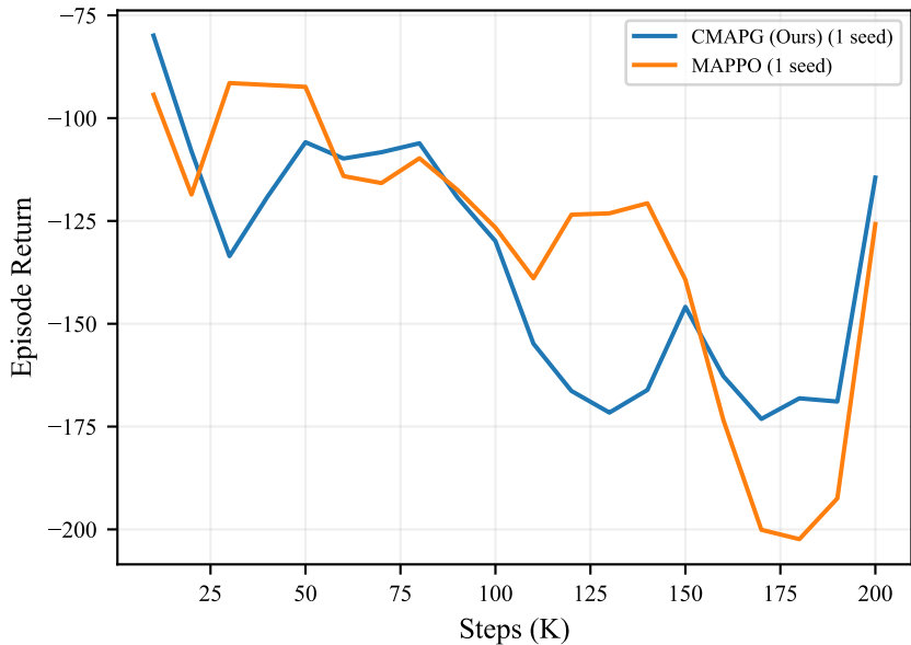
simple_spread (N=3)
