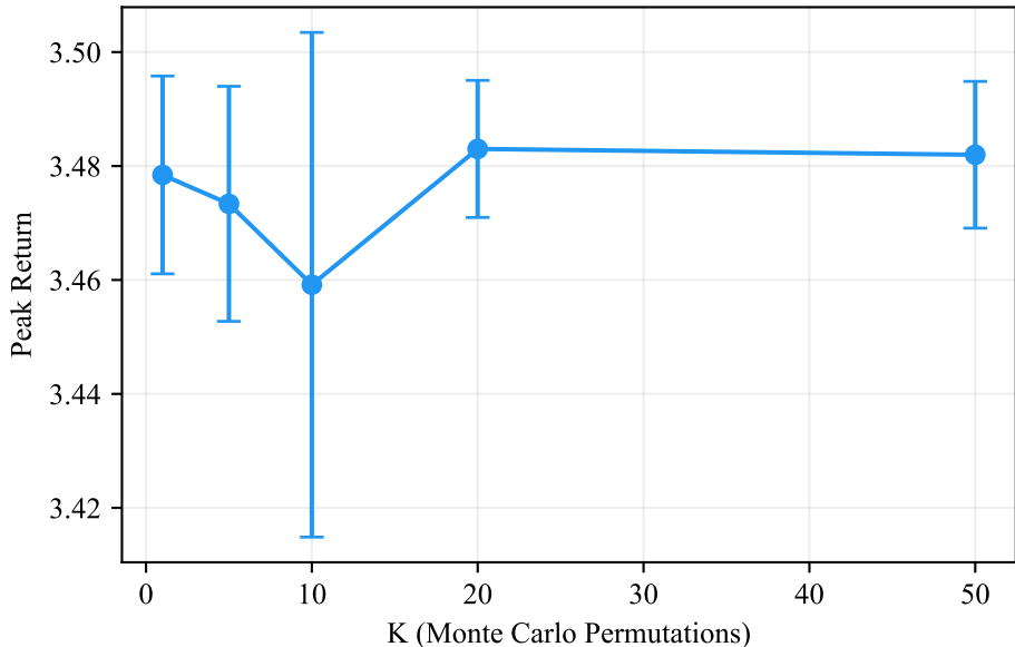
Effect of K on SVPG Performance
