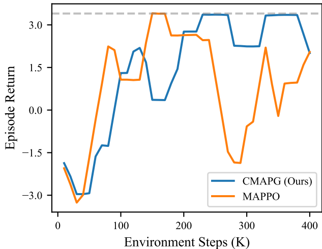
Learning Curves on Key-Lock
