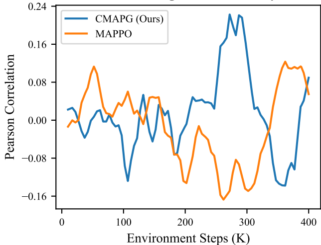
Credit Assignment Accuracy
