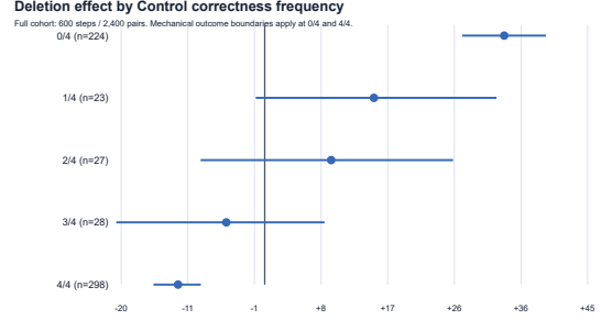
Figure 4: Deletion effect by control-run stability. Gains exist only where control already fails. Outcome-conditioned strata: conditioning on the control draws biases the extreme strata outward (regression to the mean), so these are descriptive bounds, not causal subgroup effects.
