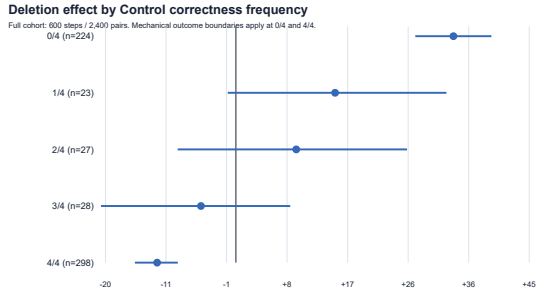
Figure 3: Deletion effect by control-run stability. Gains exist only where control already fails. Outcome-conditioned strata: conditioning on the control draws biases the extreme strata outward (regression to the mean), so these are descriptive bounds, not causal subgroup effects.
