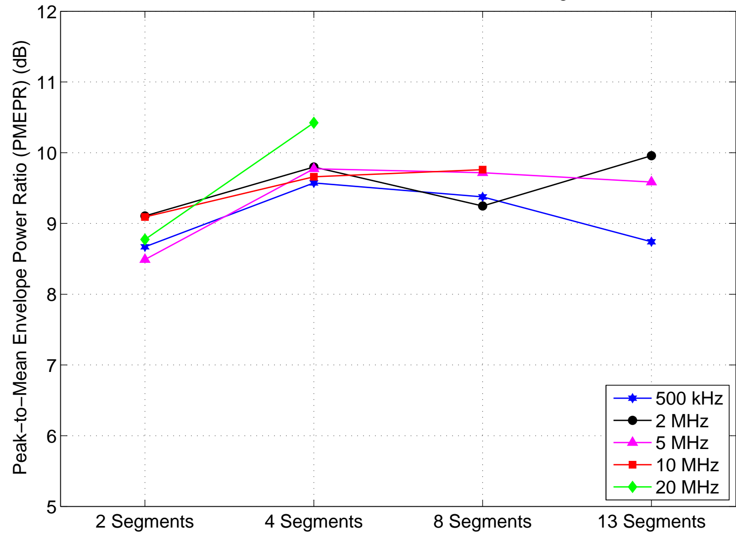
Maximum PMEPR of a 20 MHz 256QAM Signal
