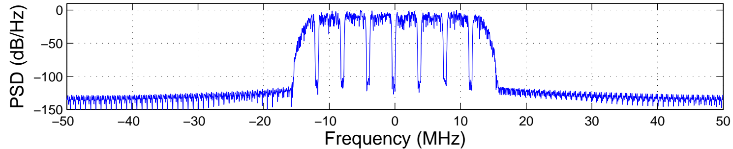
8 Segments with 500kHz Spacing
