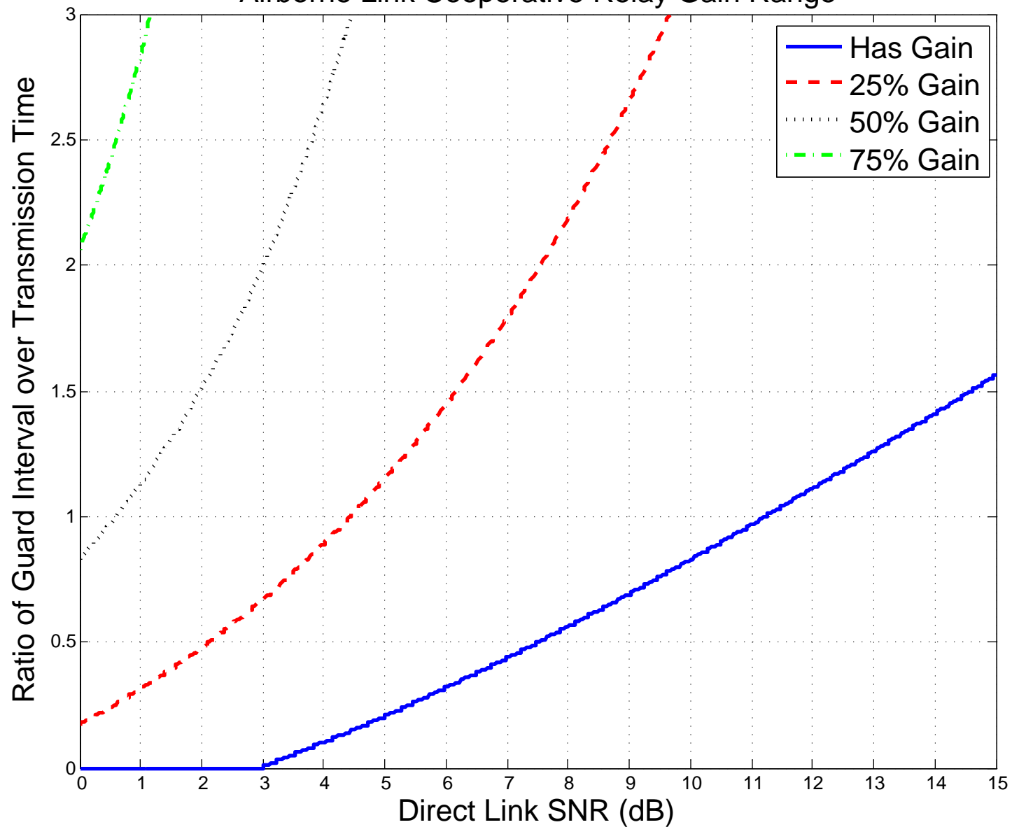
Airborne Link Cooperative Relay Gain Range
