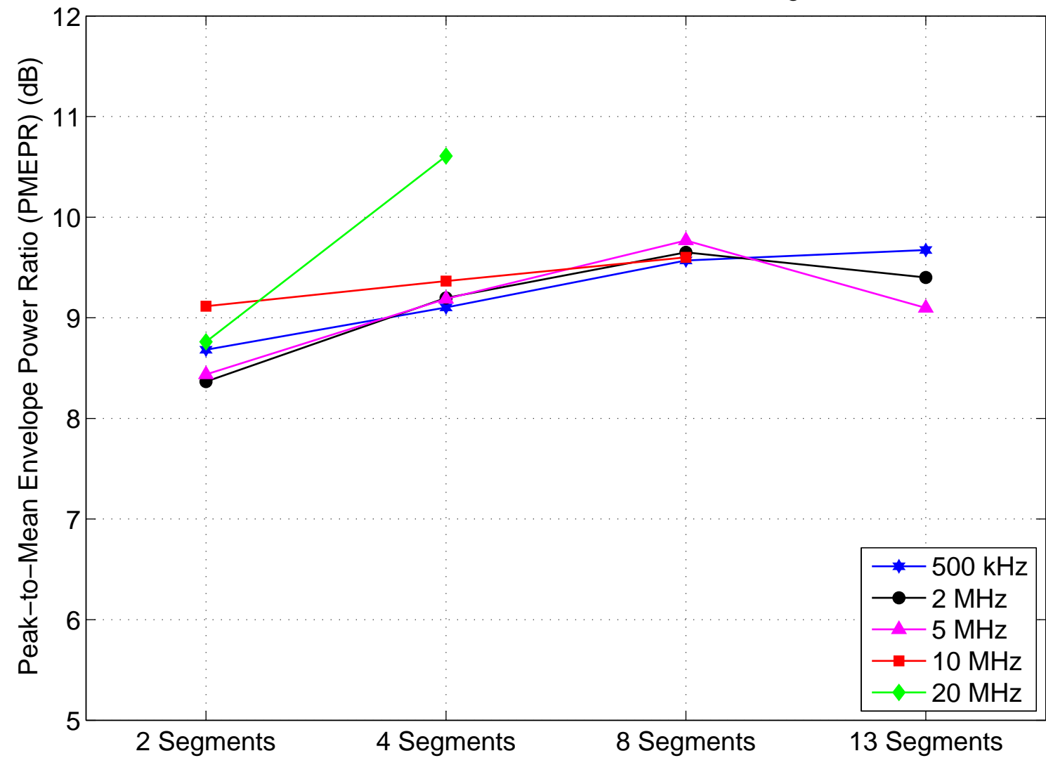
Maximum PMEPR of a 20 MHz 64QAM Signal
