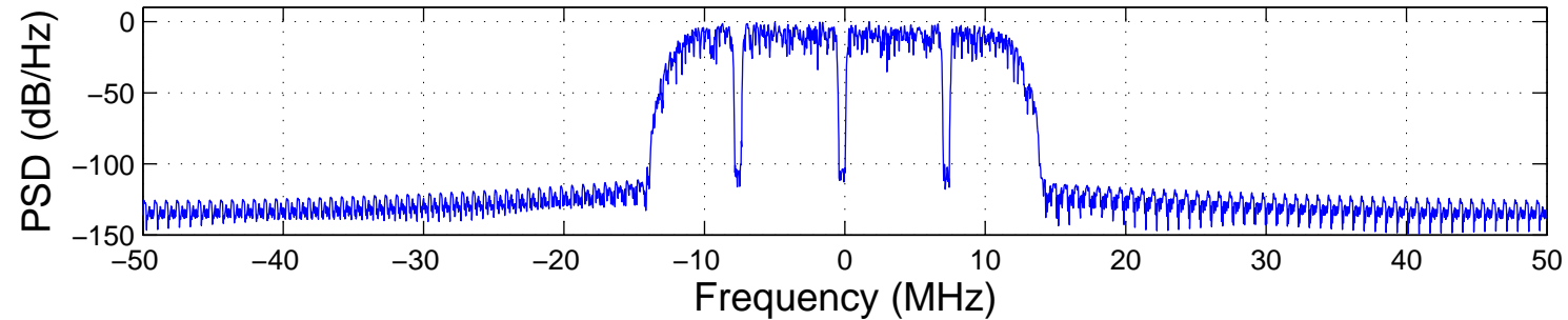
4 Segments with 500kHz Spacing
