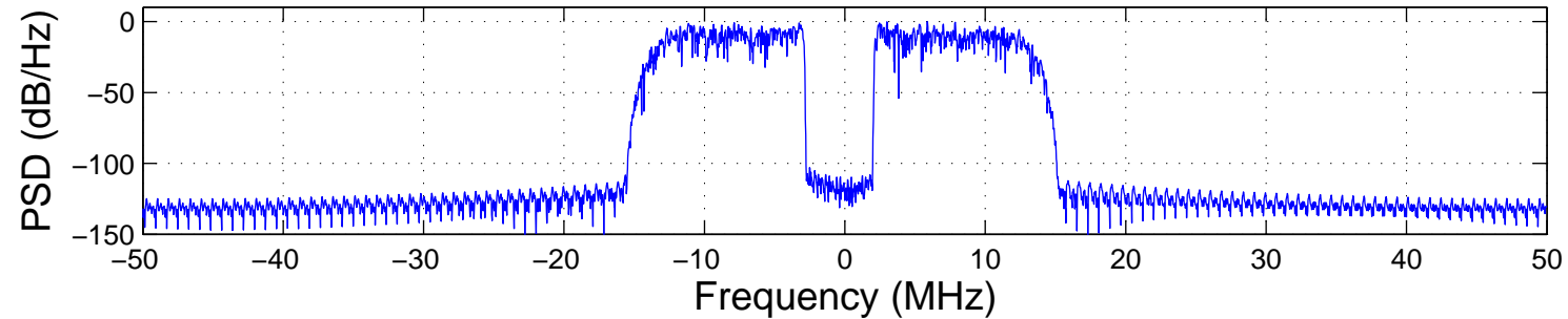
2 Segments with 5MHz Spacing
