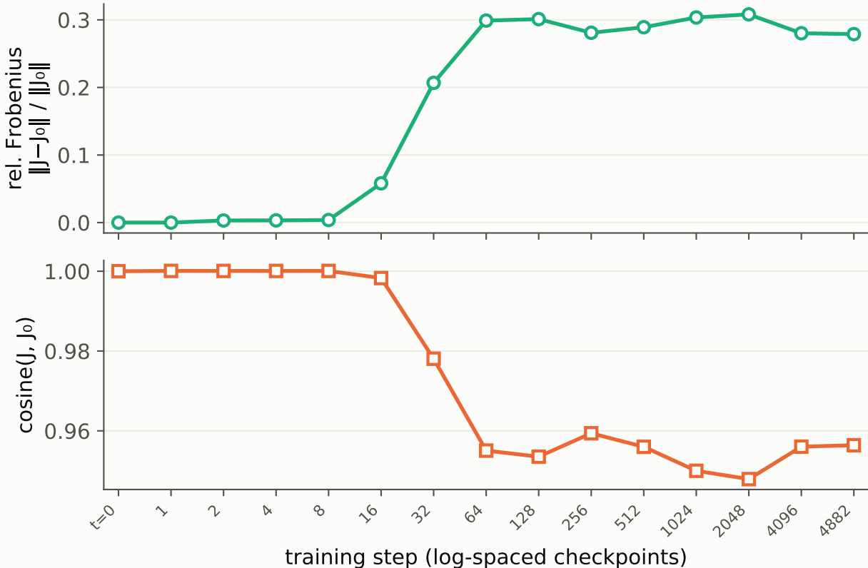
Gemma-3-1b-it — Jacobian drift from the base lens
