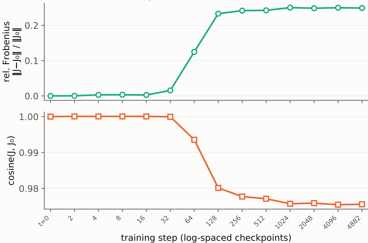
Gemma-3-270m-it — Jacobian drift from the base lens
