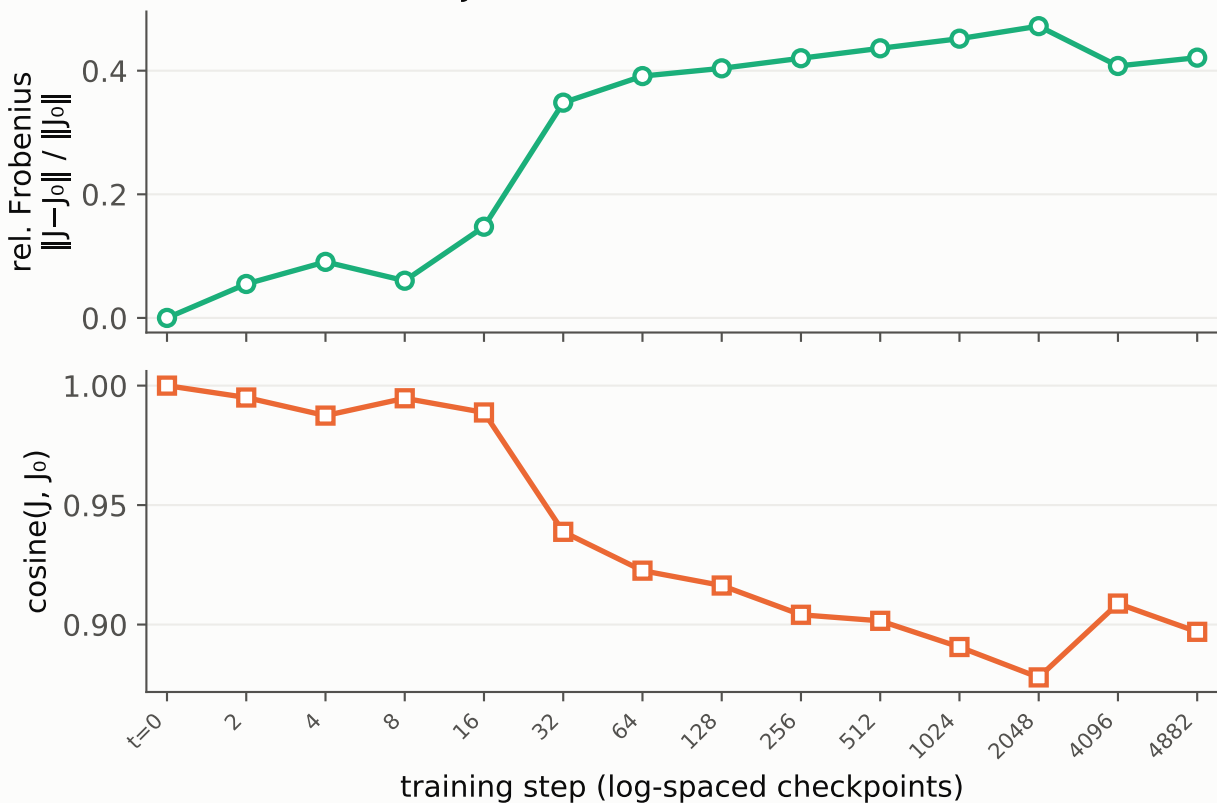
Gemma-3-12b-it — Jacobian drift from the base lens
