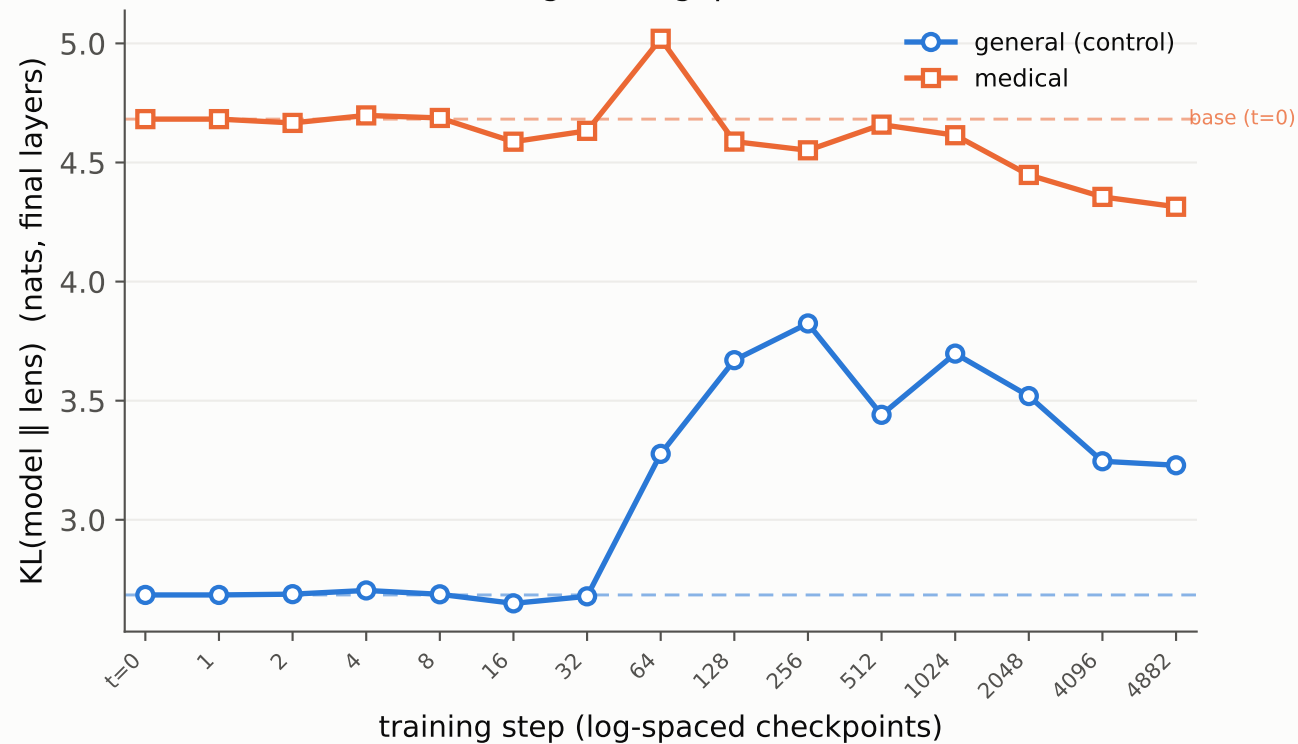
Faithfulness: the medical-general gap narrows over medical SFT
